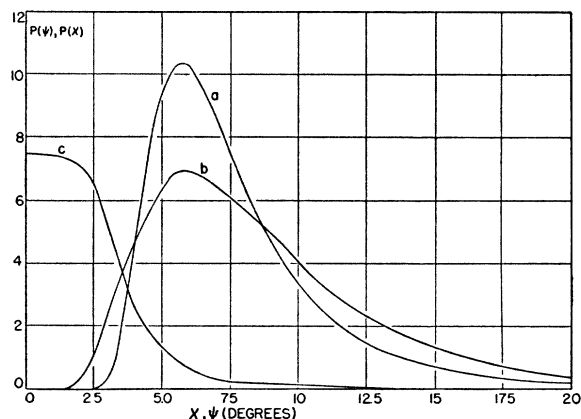
FIG. 7. Distributions in recoil angles. Curve (a): distribution in horizontal recoil angles \psi experienced by a hydrogen atom excited to the 2s state by electrons of energy just above the threshold. The temperature of the source of atoms is taken to be 2600^\circ\text{K} . The total probability would be unity if the angle were measured in radians. Curves (b) and (c): distributions in horizontal recoil angles \psi and vertical recoil angles \chi for hydrogen atoms excited to 2s by electrons of energy 13.6 ev.
