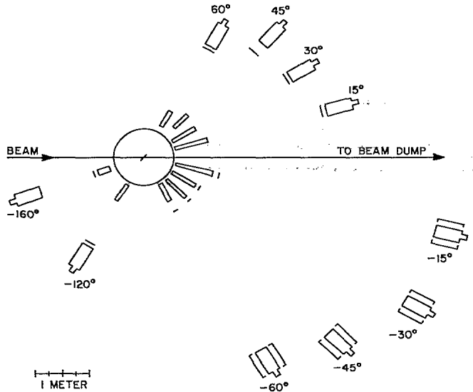
FIG. 1. Experimental setup. Groups of detectors were placed at the angles -15^\circ , -30^\circ , -45^\circ , and -60^\circ and are enclosed in brackets. Single detectors were placed at +15^\circ , +30^\circ , +45^\circ , +60^\circ , -120^\circ , and -160^\circ . The flight paths ranged from 160 to 450 cm. The rectangular boxes represent shadow bars (the -15^\circ bar is tapered), and the solid lines in front of detectors or behind shadow bars represent the proton veto paddles.
