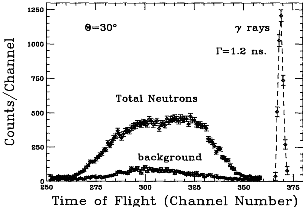
FIG. 2. Typical time-of-flight spectrum for neutrons and \gamma rays. The data for total neutrons includes target and background contributions. The background contribution is also shown separately. Subtracting the background from the total gives the target neutron. The width of the \gamma peak is 1.2 ns. The time-to-digital converter calibration is 0.2607 ns/channel.
