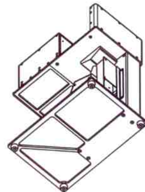
View of Experimenter's XRF Kit from the bottom
